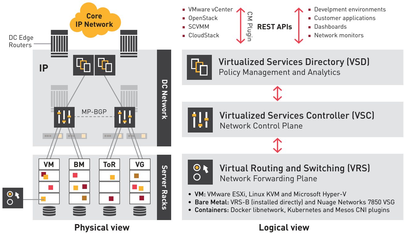
FIGURE 2. Nuage Networks Virtualized Services Platform Architecture
