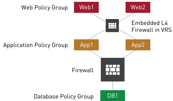
FIGURE 4. Nuage Networks VSP enforces security policies between application tiers in a virtual network with firewall features in the VRS, or by service chaining third-party security devices such as a next-generation firewall or intrusion prevention system (either physical or virtual).
