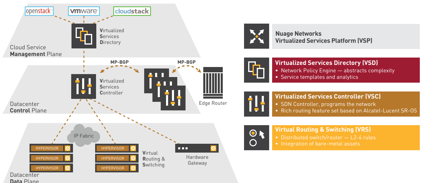
FIGURE 2. Nuage Networks VSP open and dynamic datacenter network fabric
