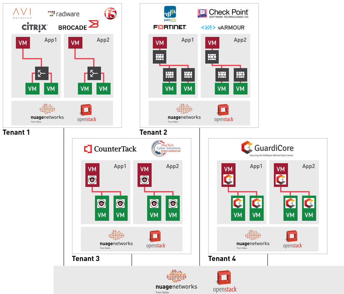
FIGURE 3. Multi-tenant isolation provided by dedicated Nuage Networks VSP instances
